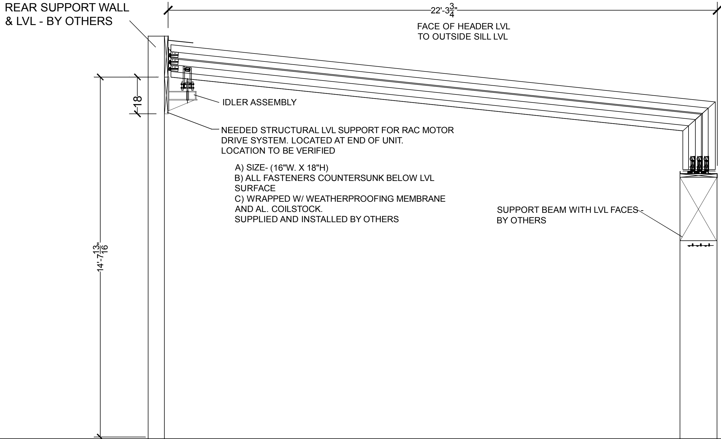
LEFT SECTION W/ OPENER
