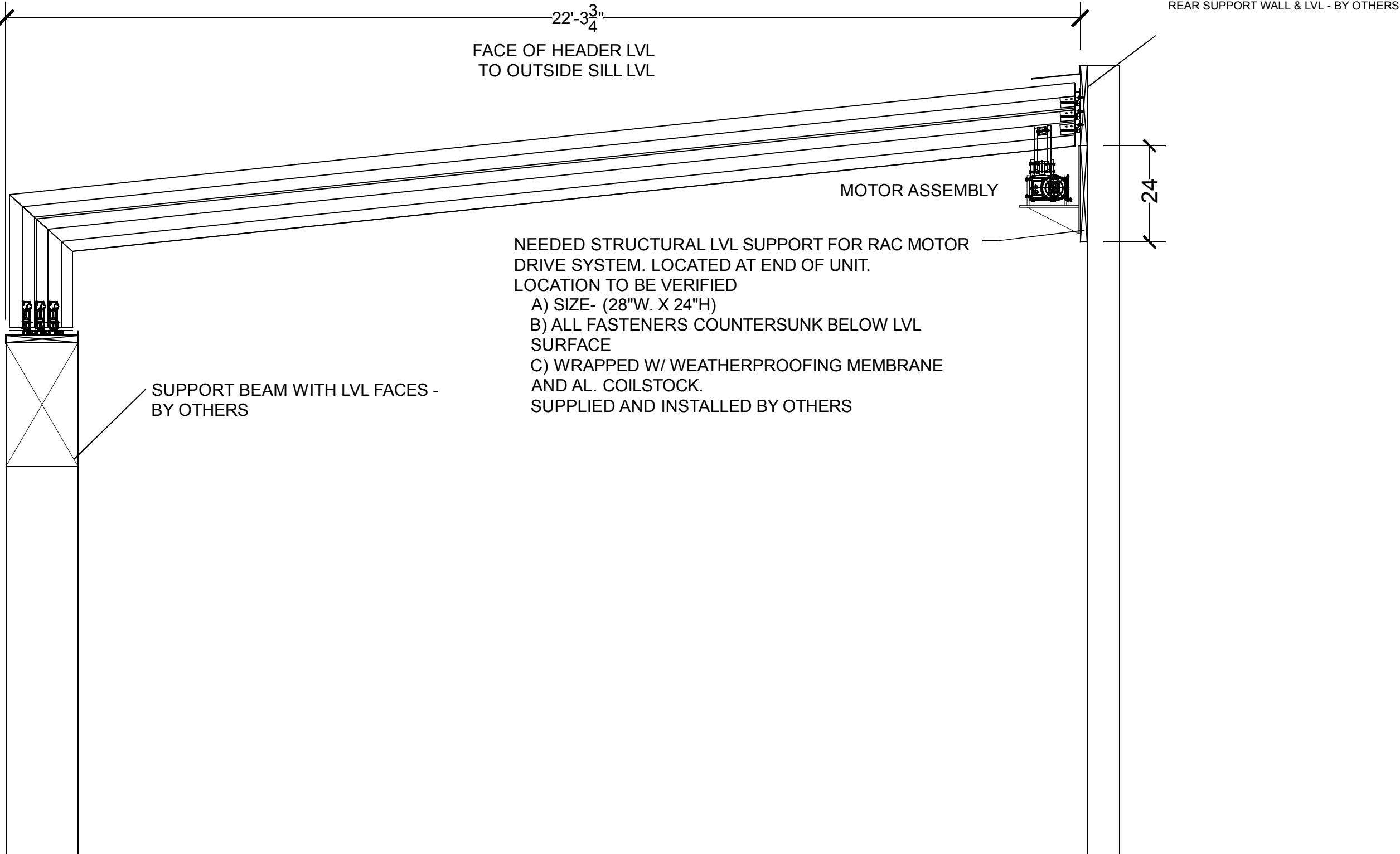
RIGHT SECTION W/ OPENER
