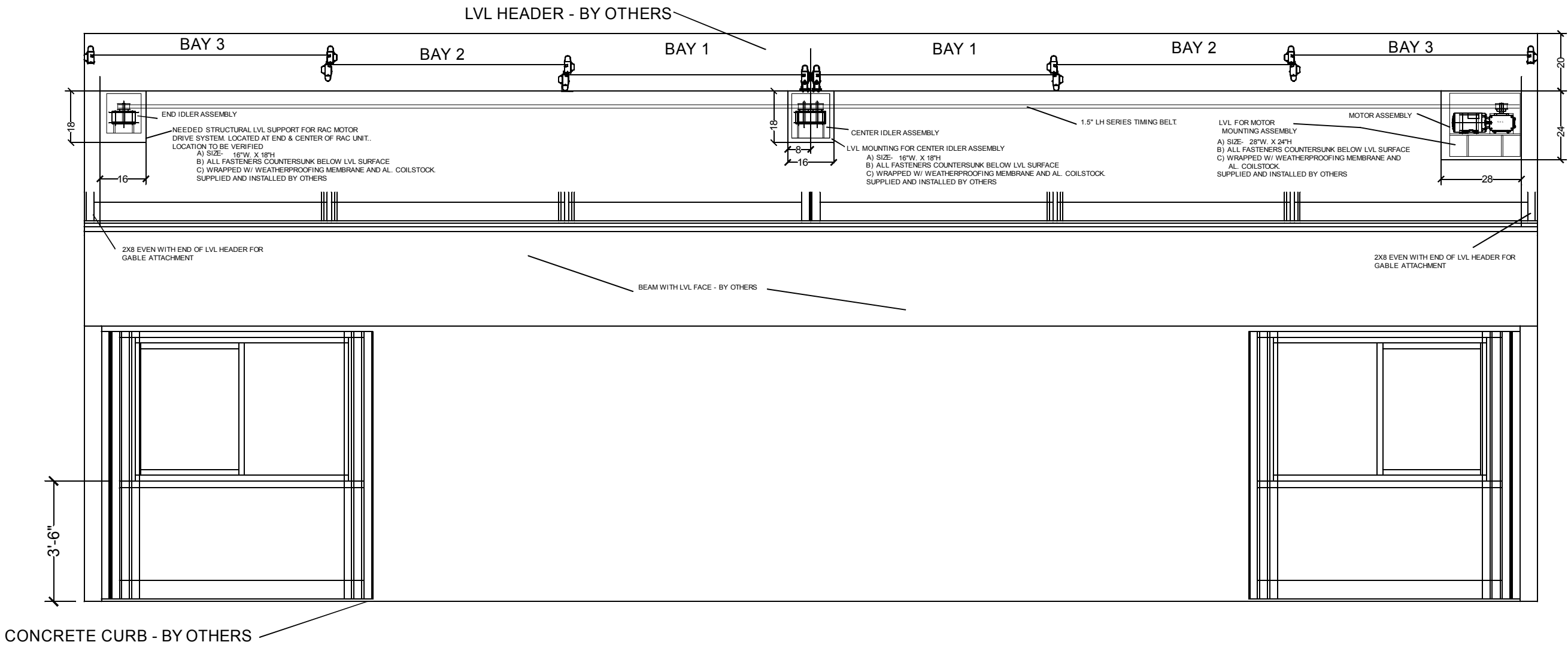
FRONT ELEVATION - OPEN W/ MOTOR
